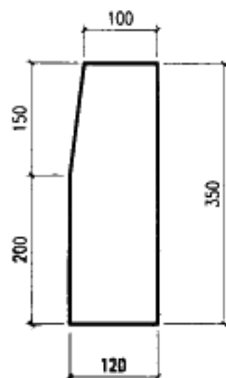
③ 混凝土立缘石 (100/120X350X495)
