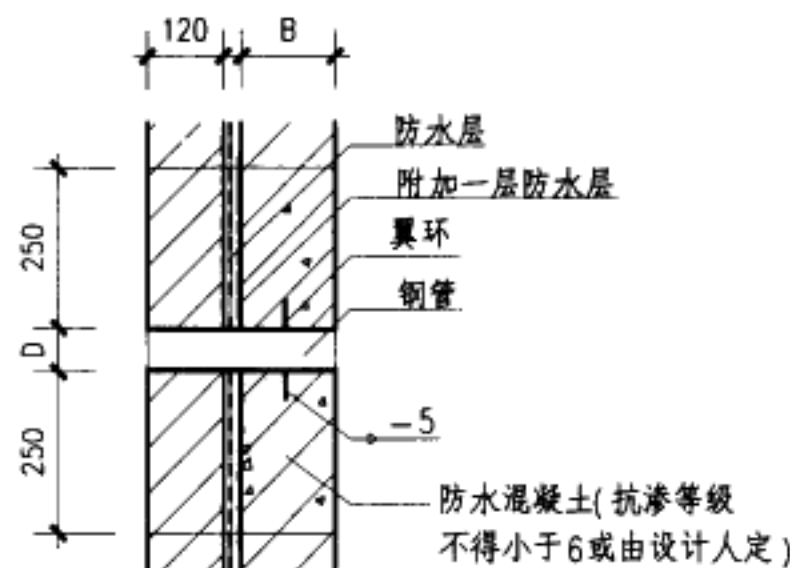
2 预留洞翼环式管道穿池壁
