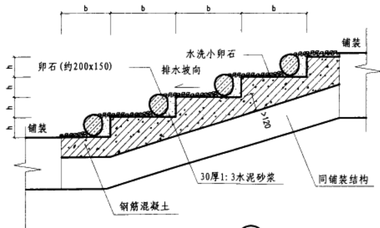
③ 卵石砌台台阶
